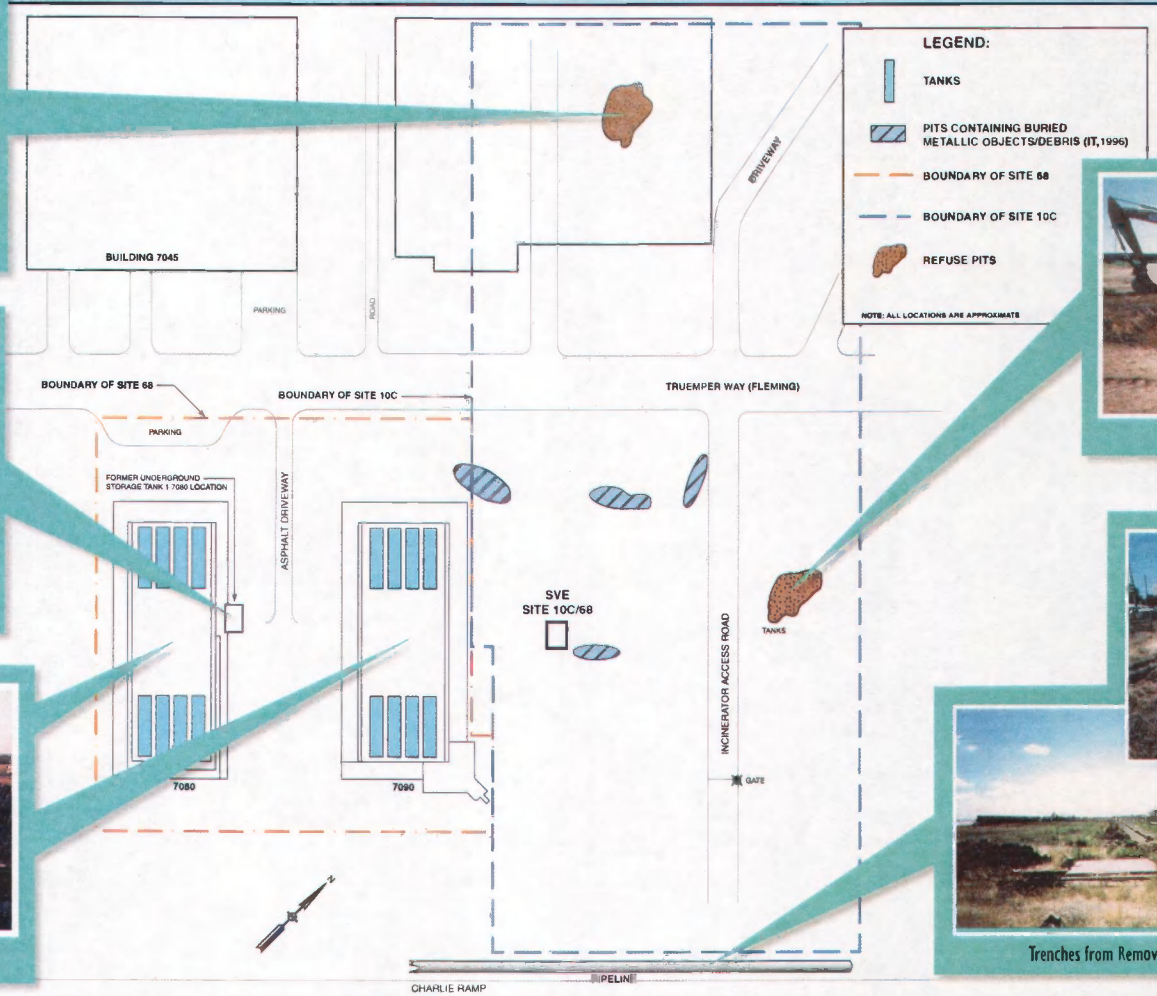
Backfilling of Excavation Pits 7080 and 7090
